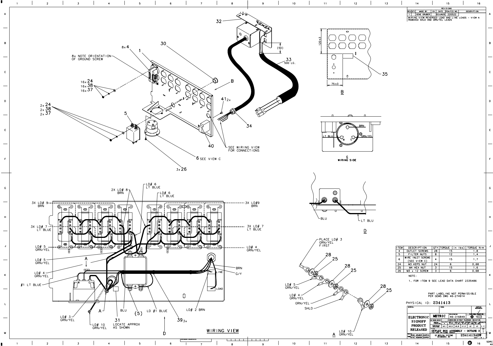
Figure 6-26 Outlet Box Assembly (2341413, sheet 1, rev 1)
