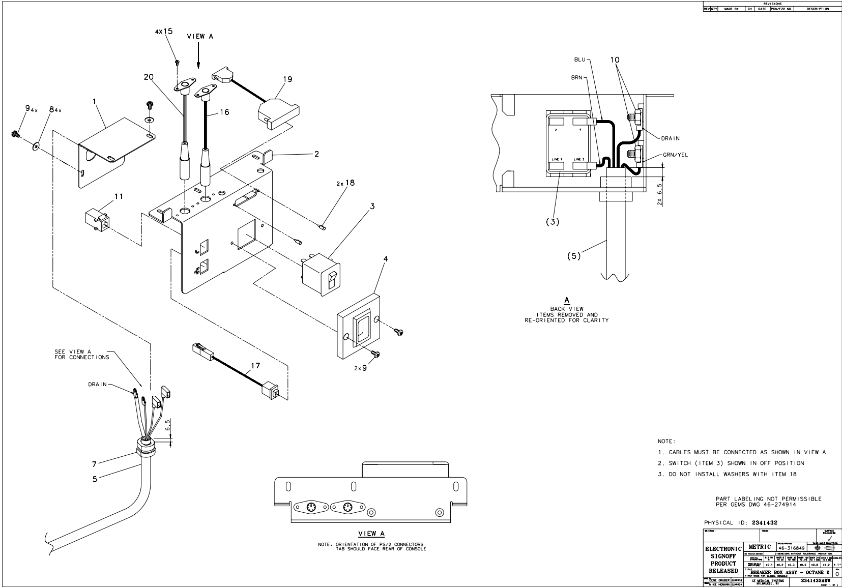
Figure 6-27 Breaker Assembly (2341432, sheet 1, rev 0)
