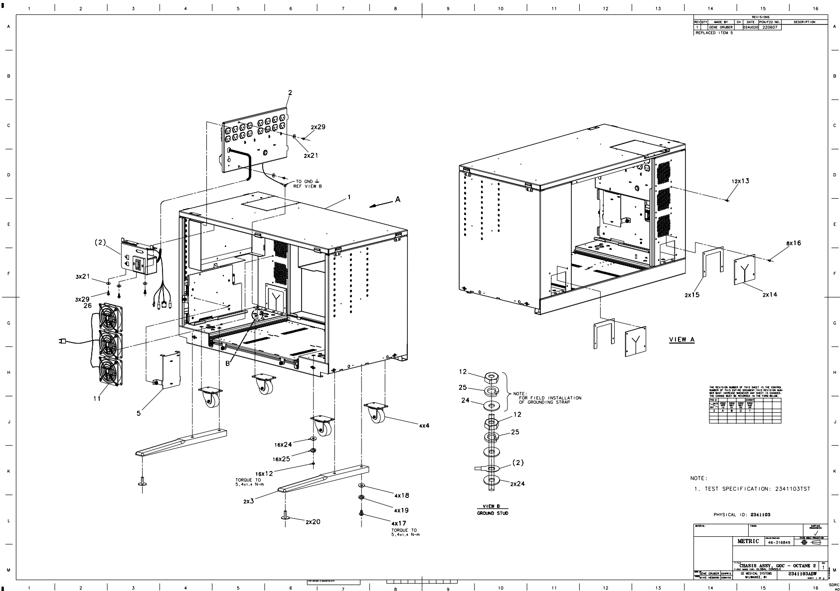
Figure 6-24 Console Chassis Assembly (2341103, sheet 1, rev 1)
