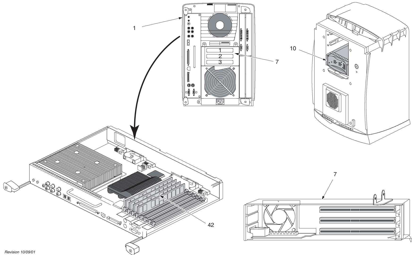
Figure 6-9 Octane2 Replacement Parts (sheet 1, rev 10/09/01)
