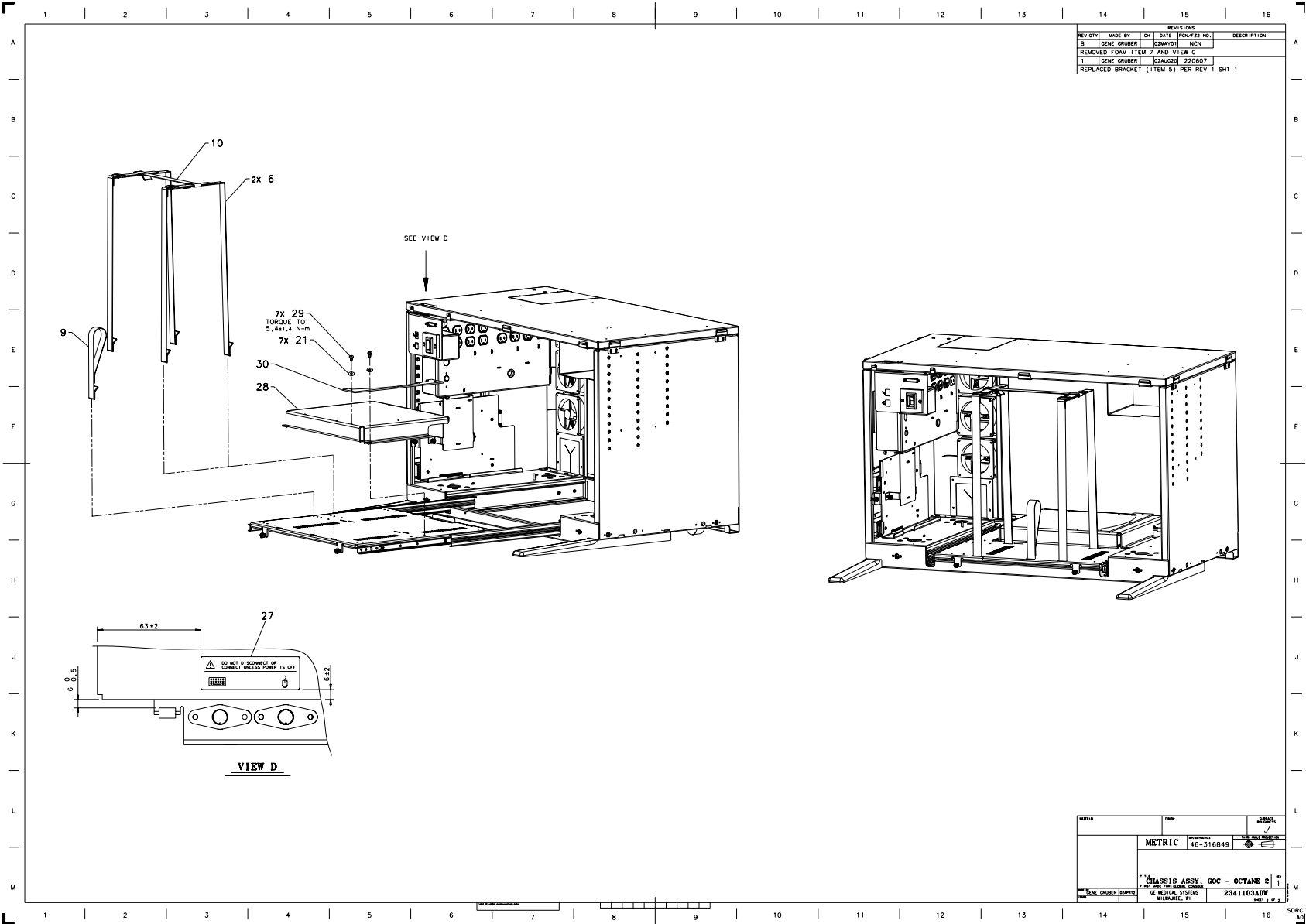
Figure 6-25 Console Chassis Assembly (2341103, sheet 2, rev 1)
