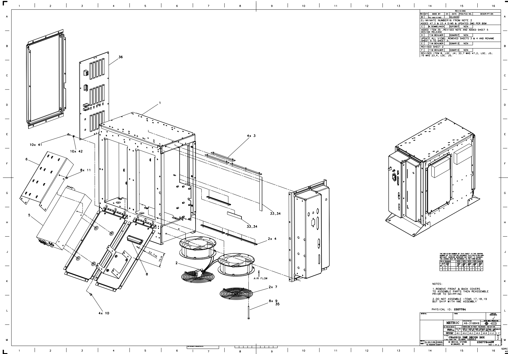
Figure 6-17 VME Chassis Assembly (2307794, sheet 1, rev 2)
