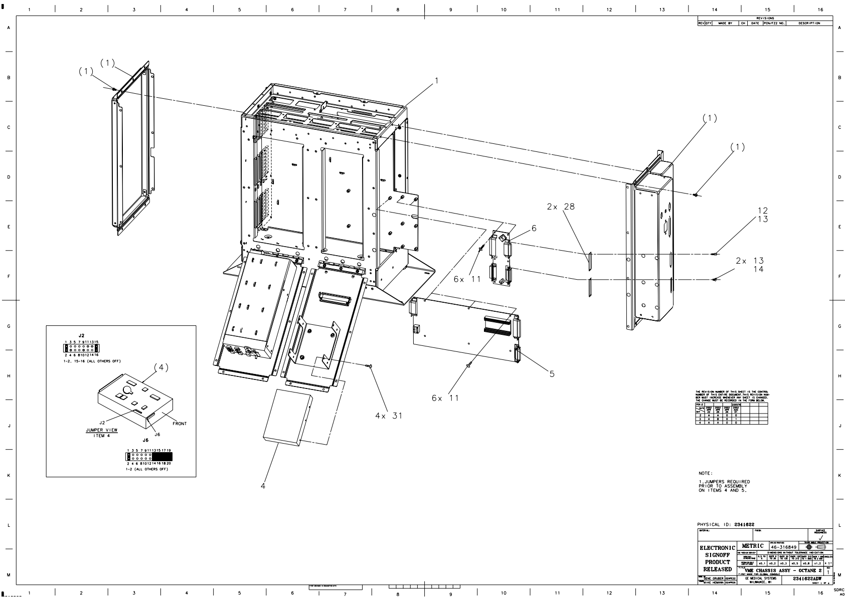
Figure 6-10 VME Recon Engine Assembly (2341622, sheet 1, rev 1)
