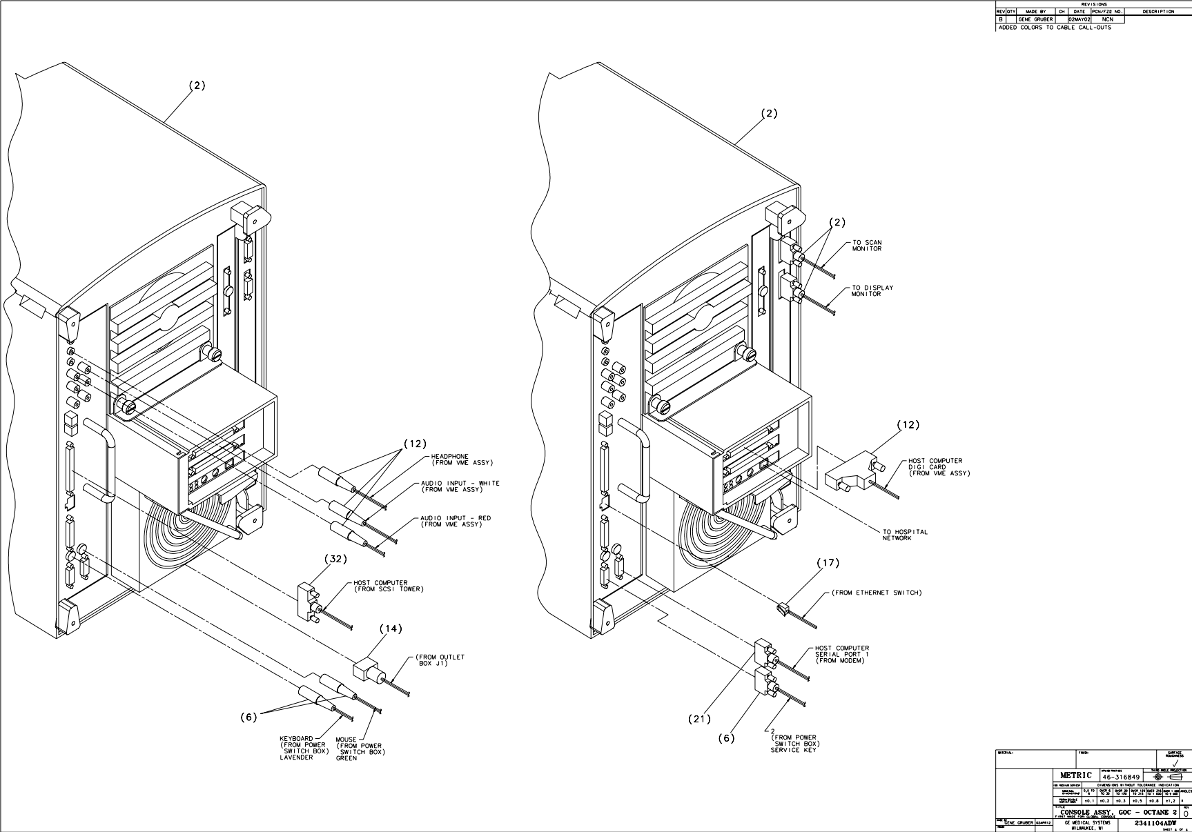
Figure 6-5 Console GOC1-Octane2 (2341104, sheet 4, rev 0)
