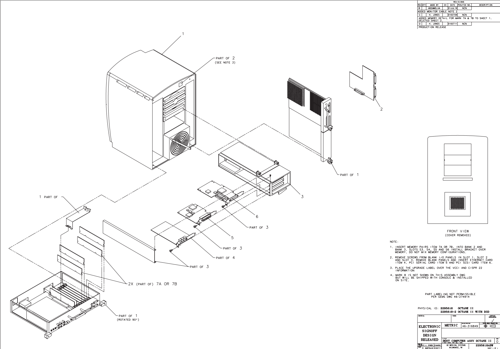
Figure 6-8 Octane2 Computer Assembly (2295618, sheet 1, rev 0)
