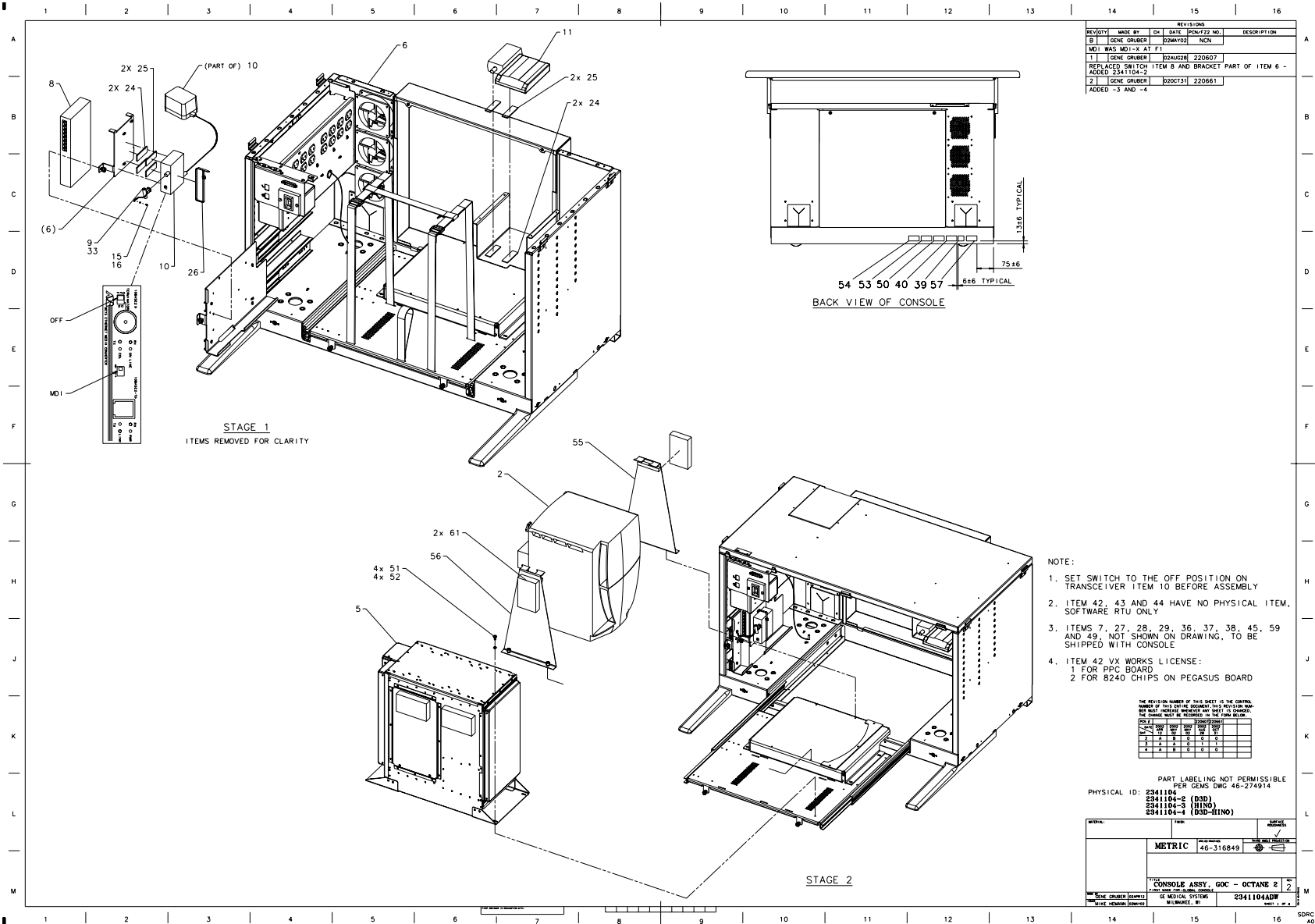
Figure 6-2 Console, GOC1-Octane2 (2341104, sheet 1, rev 2)
