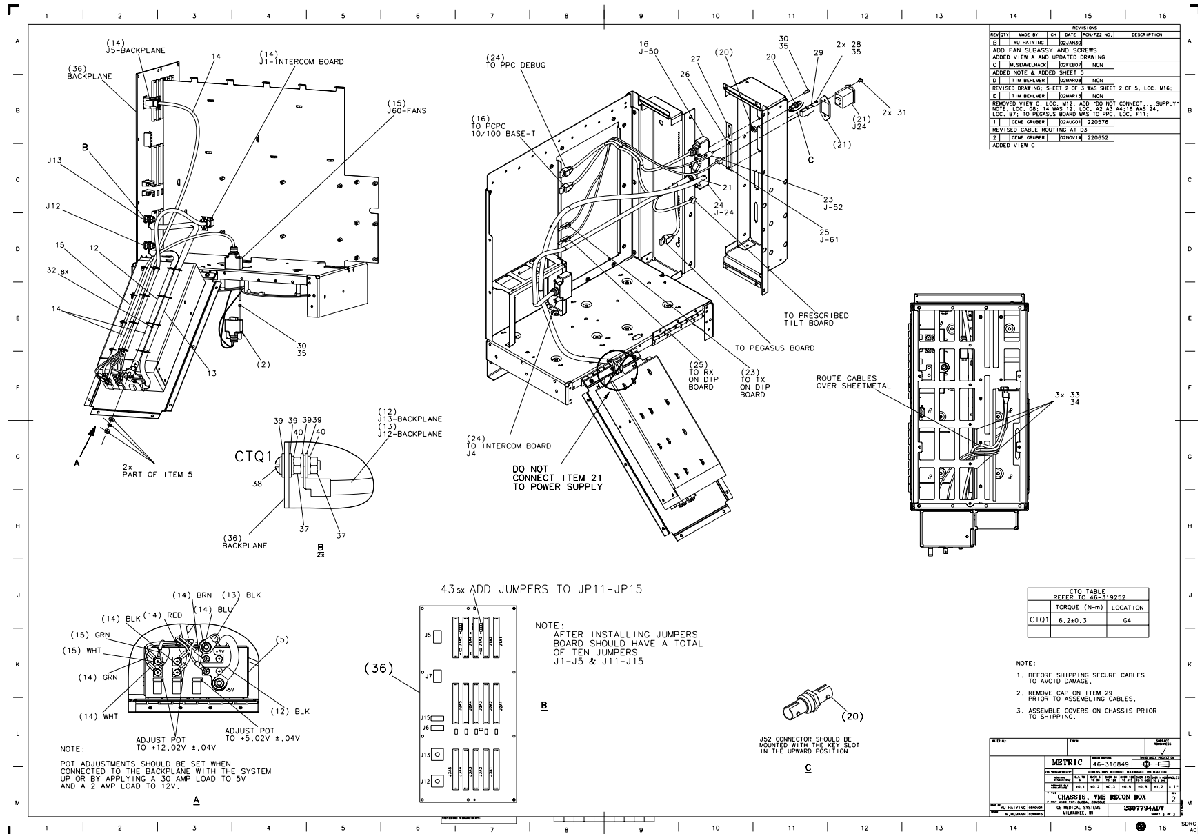
Figure 6-18 VME Chassis Assembly (2307794, sheet 2, rev 2)
