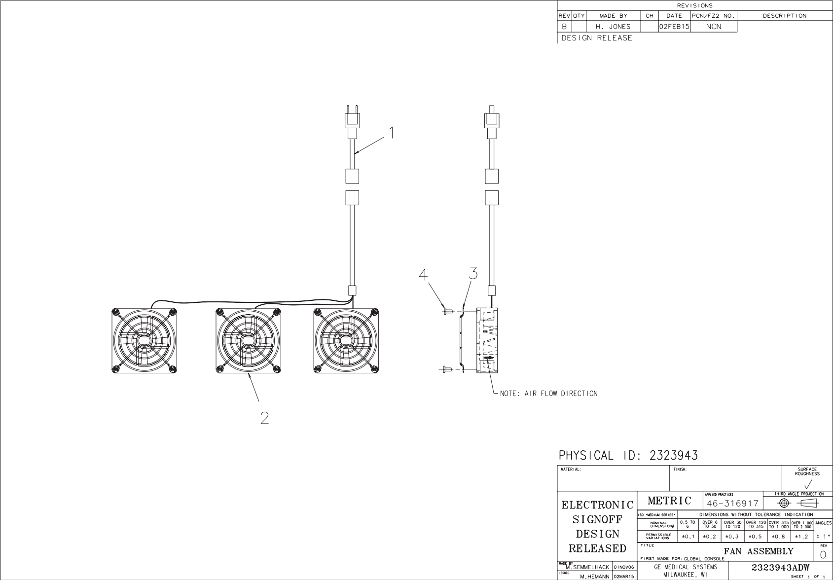
Figure 6-28 Fan Assembly, Console Chassis (2323943, sheet 1, rev 0)
