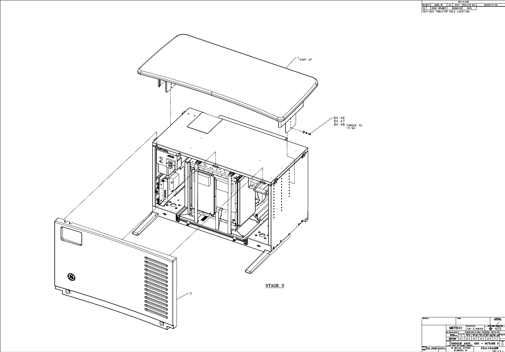
Figure 6-3 Console GOC1-Octane2 (2341104, sheet 2, rev 0)
